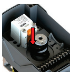
Fig. 4: Cam setting
